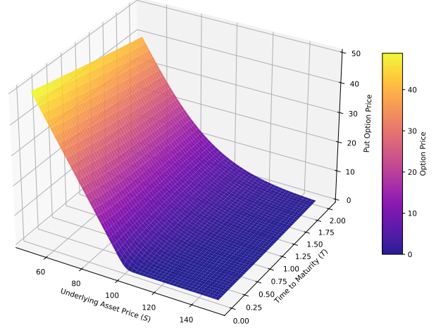
Figure 2. Black-Scholes option-price surfaces over asset price and time to maturity. The terminal payoff kink is smoothed backward in time by the diffusion structure of the PDE, producing a continuous continuation-value surface.
