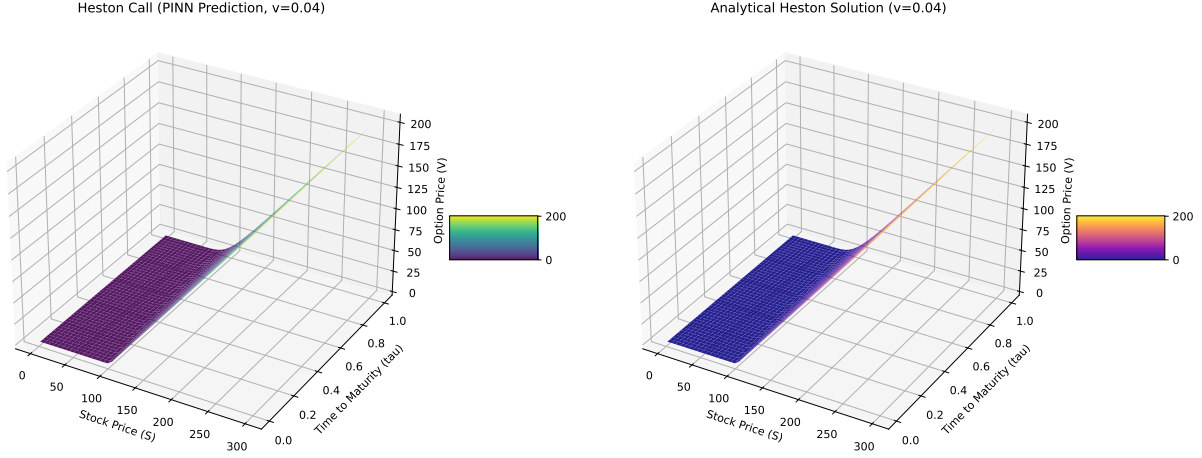
Figure 6. Final Heston PINN after 50,000 epochs on the variance slice v = v_0 = 0.04 , compared with the semi-analytical Heston benchmark obtained by adaptive Gauss–Kronrod quadrature of the characteristic-function representation (7) (Heston 1993). The plotted slice is one cross-section of a three-dimensional learned surface.
