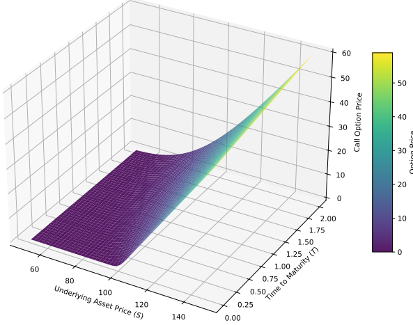
Figure 2. Black-Scholes option-price surfaces over asset price and time to maturity. The terminal payoff kink is smoothed backward in time by the diffusion structure of the PDE, producing a continuous continuation-value surface.
