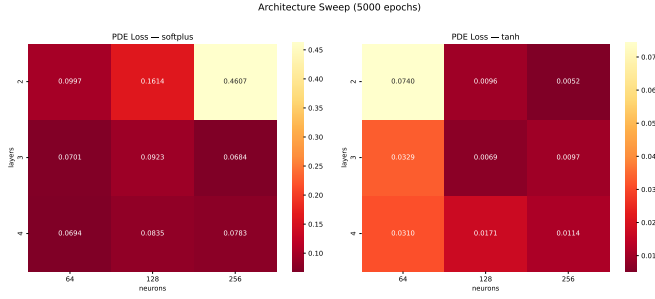
Figure 3. Black-Scholes architecture sweep after 5000 epochs (final PDE residual loss). tanh activations dominate softplus at every (depth,width) pair, and the best configuration is the wide-shallow 2 \times 256 tanh network used in the final run.
