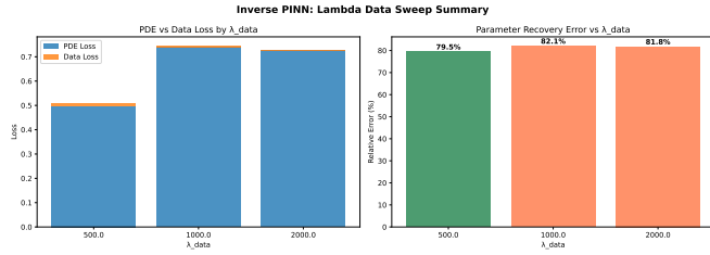
Figure 7. Inverse-PINN \lambda_{data} sweep. Left: PDE and data losses across the three weights. Right: relative parameter recovery error against truth. The lowest data loss is at \lambda_{data} = 2000 , but the lowest parameter error is at \lambda_{data} = 500 , so price fit and structural recovery are anti-correlated here.
