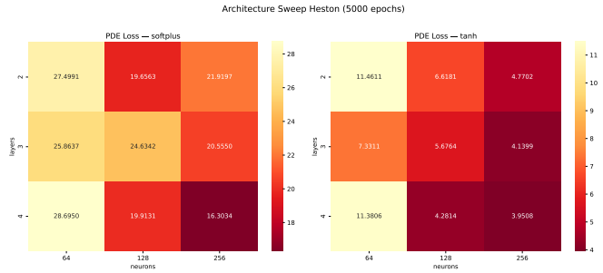
Figure 5. Heston architecture sweep after 5000 epochs. tanh networks again dominate softplus ; depth matters more than for Black-Scholes because the variance direction and the mixed derivative each introduce extra second-order terms in the residual.
