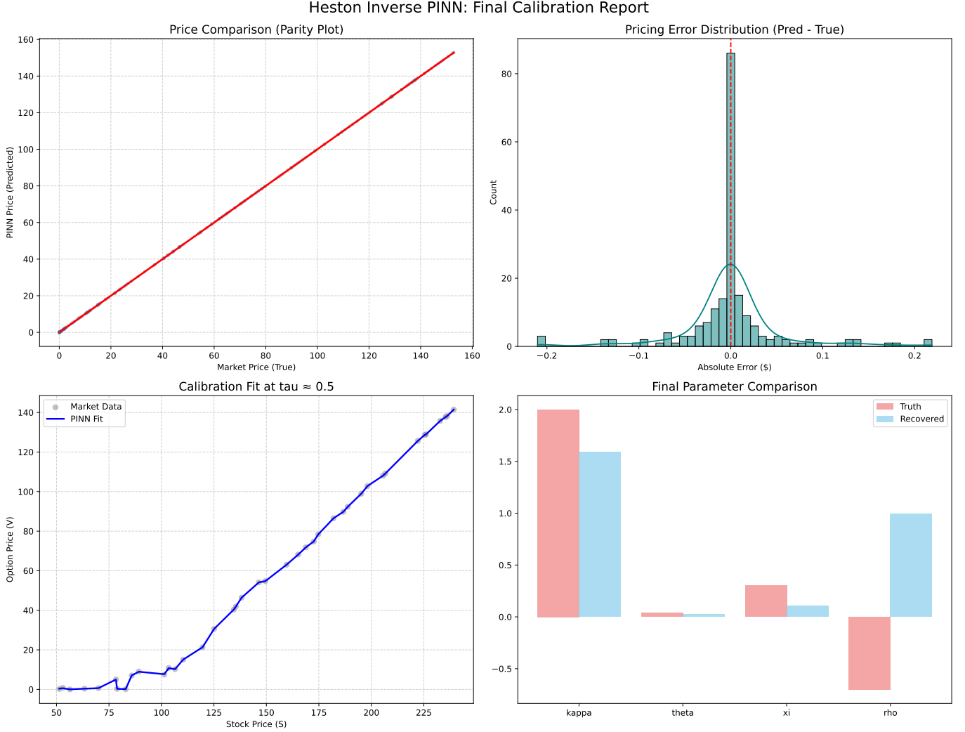
Figure 15. Final inverse Heston PINN calibration diagnostics. The figure shows strong price fit but weak structural recovery: predicted prices match the synthetic market prices closely, while the recovered Heston parameters remain biased and \rho converges to the wrong sign.
